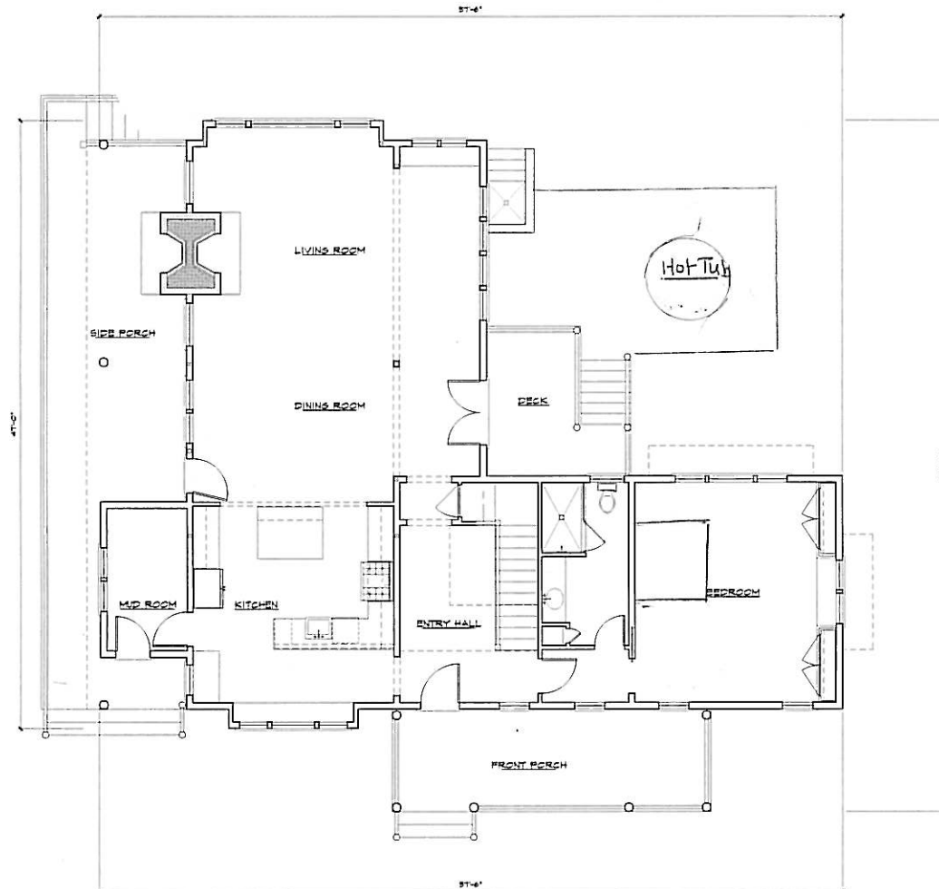
1 FIRST FLOOR PLAN ALL 1/4" = 1'-0"
